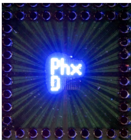
Micro-LED array integrated onto a printed circuit board during operation in full-light emission mode (left) and during display mode showing the letters "PhxD" (right). The pixel size is 30 micrometres, comparable to smartphone displays, but with much brighter light and a faster switch-on time. In combination with advanced colour converters, new mass transfer technologies are needed to accomplish even smaller and multicolour pixels. We develop the manufacturing processes required to realize micro-LED modules, focusing on reliability, high throughput and cost-effectiveness.
