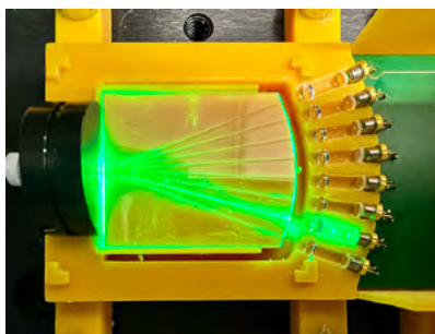
Printed waveguides.
