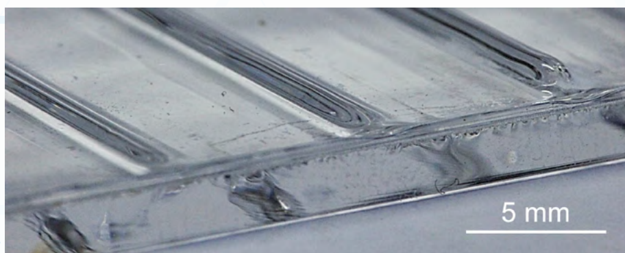
Printed transparent fused silica structures consisting of one, two and four layers (from left to right) without boundary layers.
